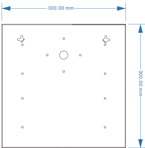
Rear panel-back
