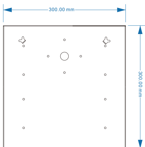
Rear panel-back
