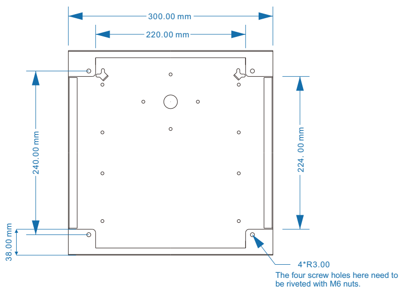
Rear panel-front
